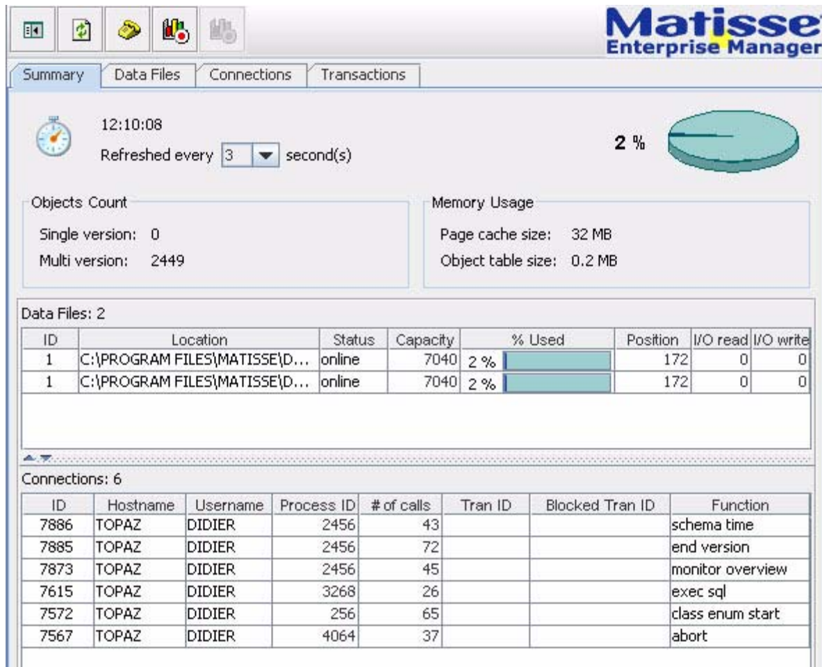
Figure 7.10 Matisse Monitoring:
