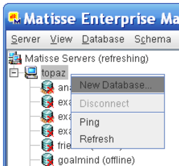
Figure 7.1 Create Database
